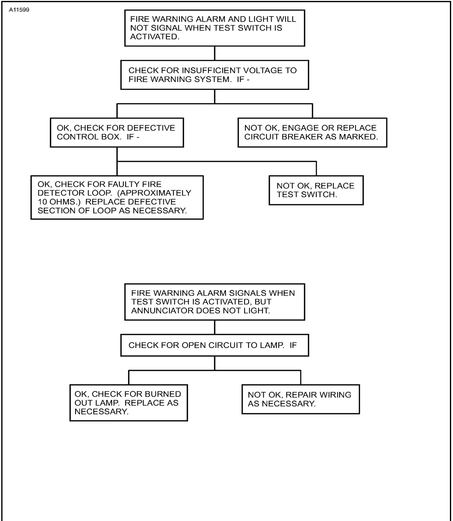
Figure 101 : Sheet 2 : Fire Detection System Troubleshooting Chart
